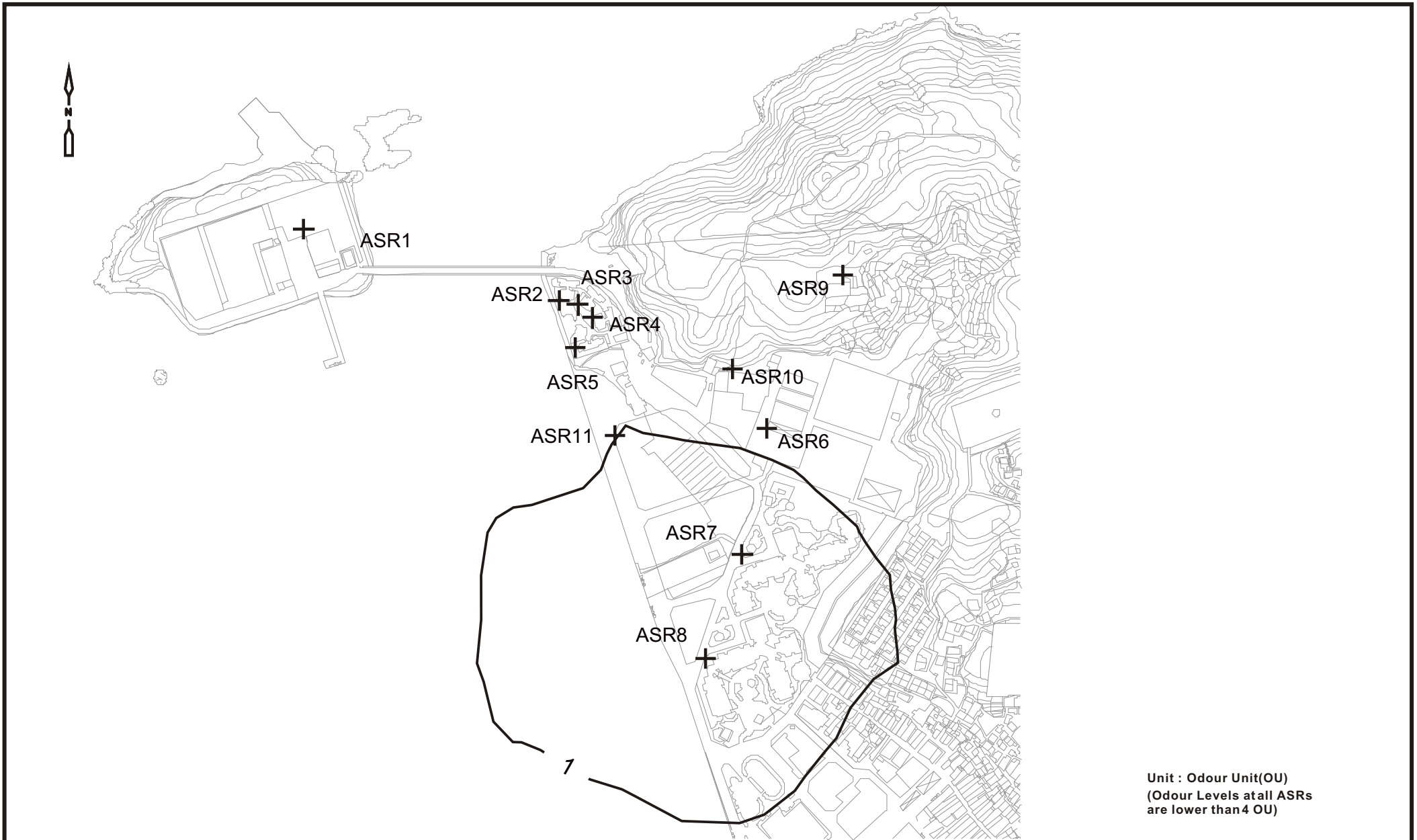
Figure 3-12 Mitigated Scenario (when Drying Bed is used) Worst 5-second Odour Level Contours Plot (10m Above Ground Level)
